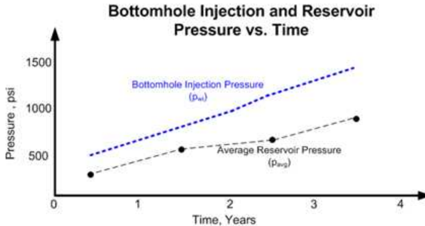
Figure 2. Sandface (bottomhole) injection and reservoir pressure vs. time
