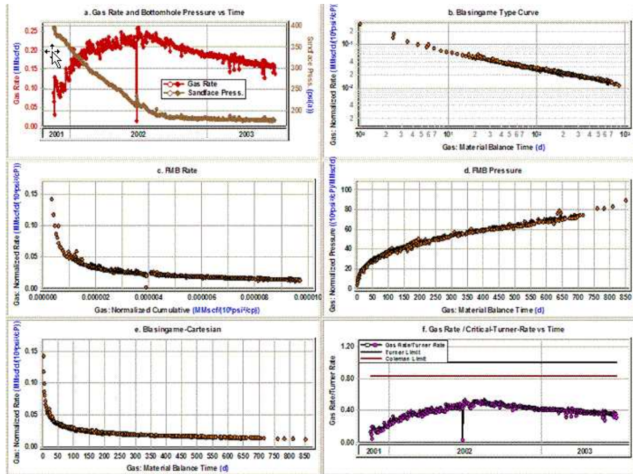
Figure 6: Case 5 diagnostic plots
