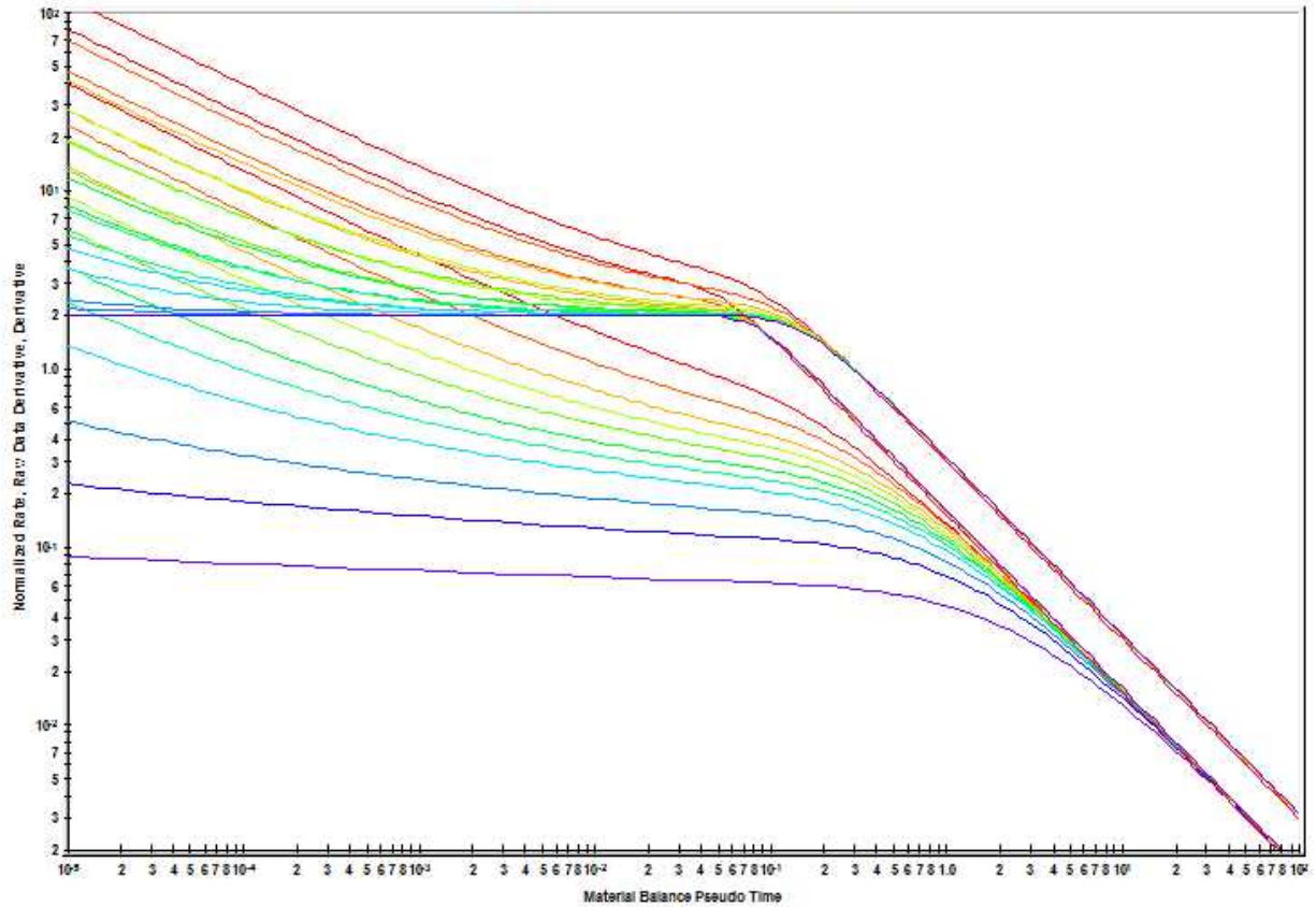
Agarwal-Gardner Typecurve Analysis
