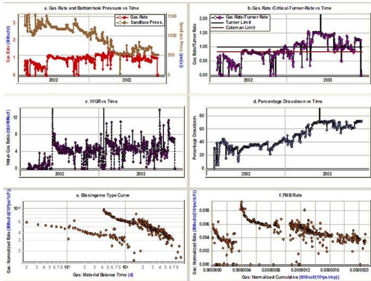
Figure 5: Case 4 diagnostic plots
